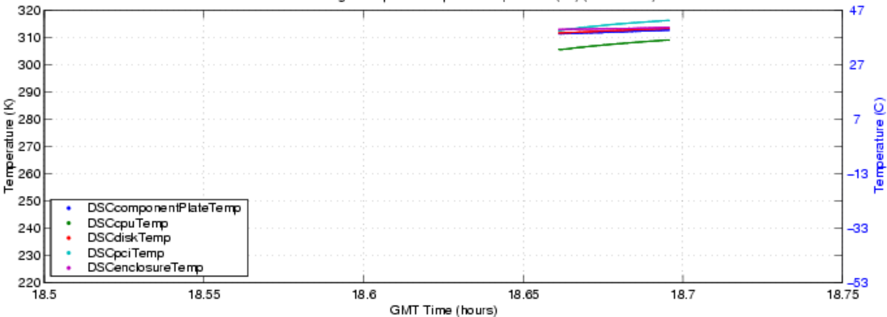
S-HIS Data Storage Computer Temperatures , 050607 (fbf) (ENG Plot 8)
