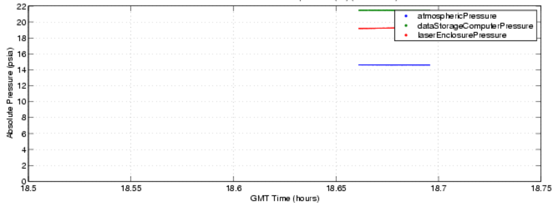
S-HIS Environmental Parameters, 050607 (fbf) (ENG Plot 8)
