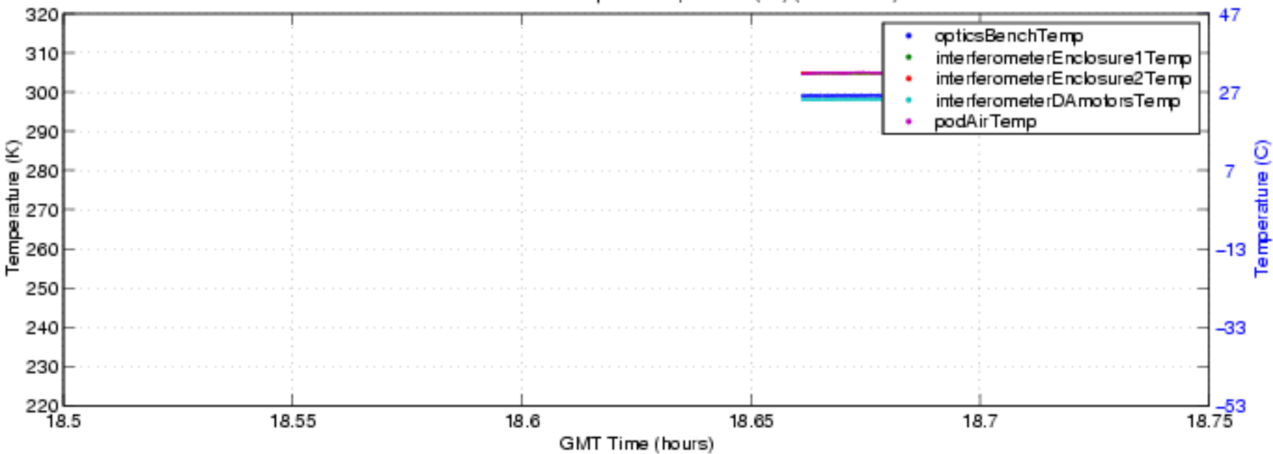
S-HIS Interferometer Temperatures, 050607 (bf) (ENG Plot 5)
