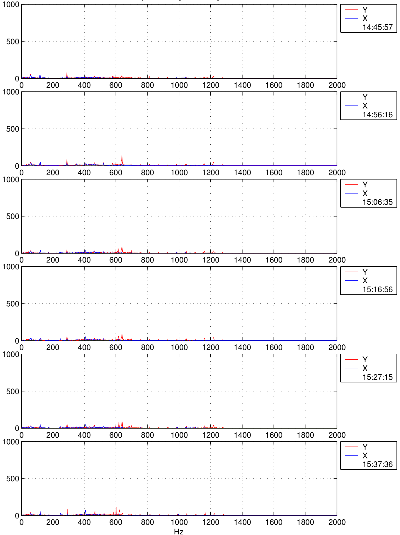
DA Tilt Error Angle Power Spectrum Number of samples averaged: 10; flight date: 050606
