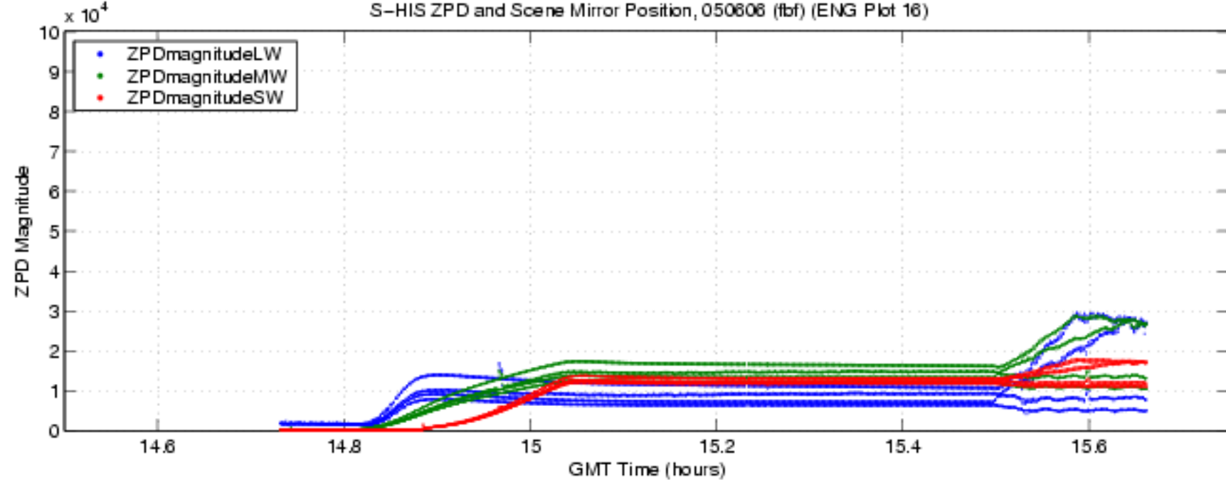
S-HIS ZPD and Scene Mirror Position, 050606 (fbf) (ENG Plot 16)
