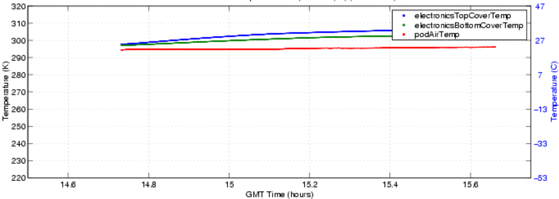
S-HIS Electronics Temperatures 2/2, 050606 (fbf) (ENG Plot 8)
