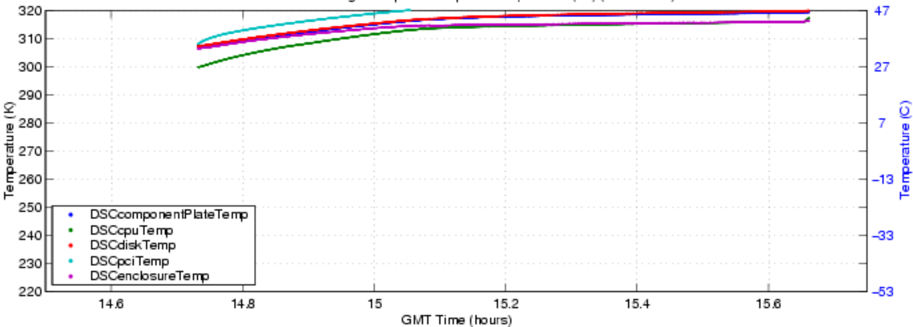
S-HIS Data Storage Computer Temperatures , 050606 (fbf) (ENG Plot 8)
