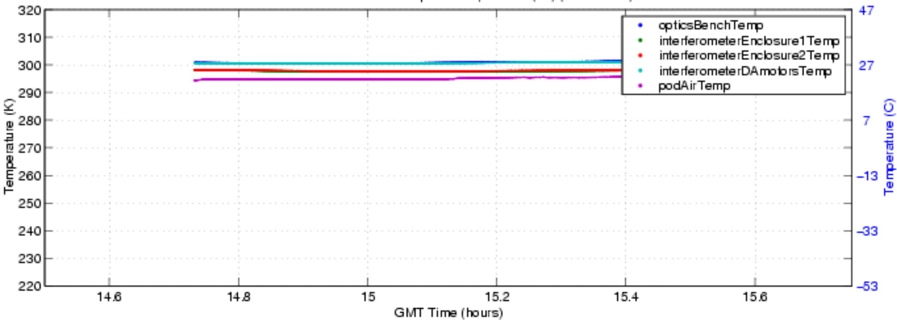
S-HIS Interferometer Temperatures, 050606 (bf) (ENG Plot 5)
