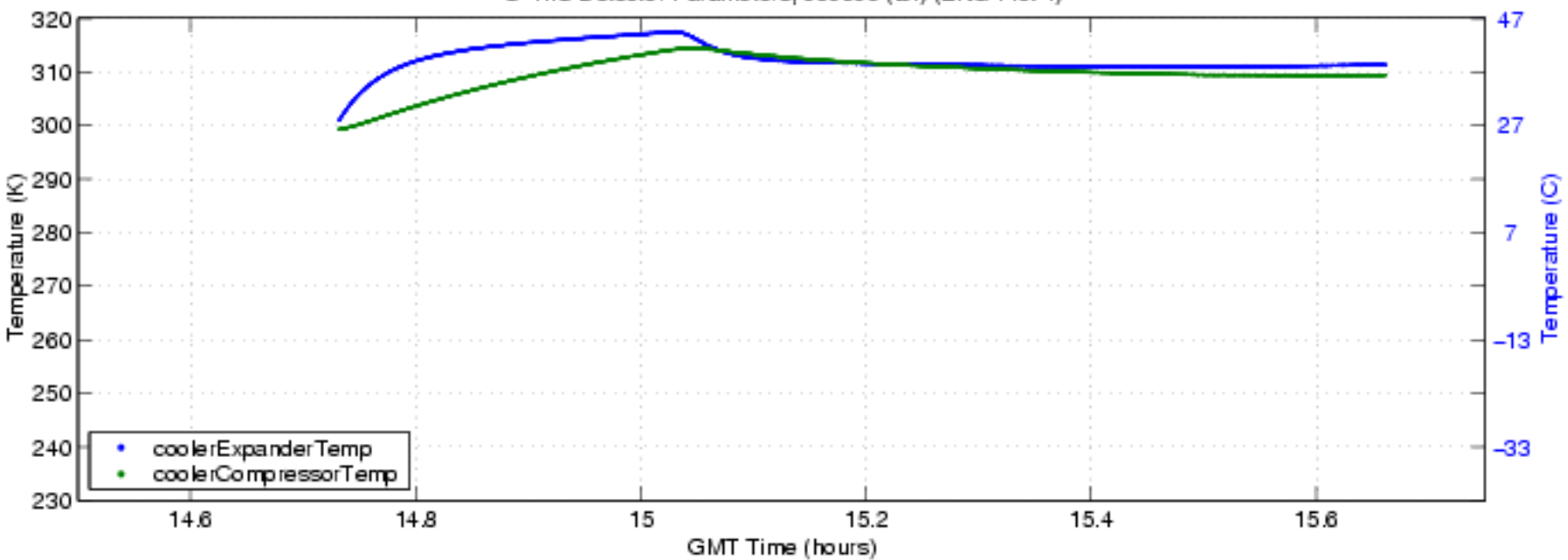
S-HIS Detector Parameters, 050606 (bf) (ENG Plot 4)
