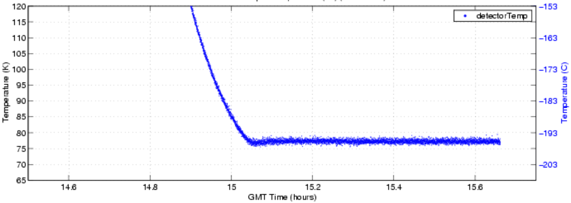
S-HIS Detector Temperature, 050606 (fbf) (ENG Plot 3)
