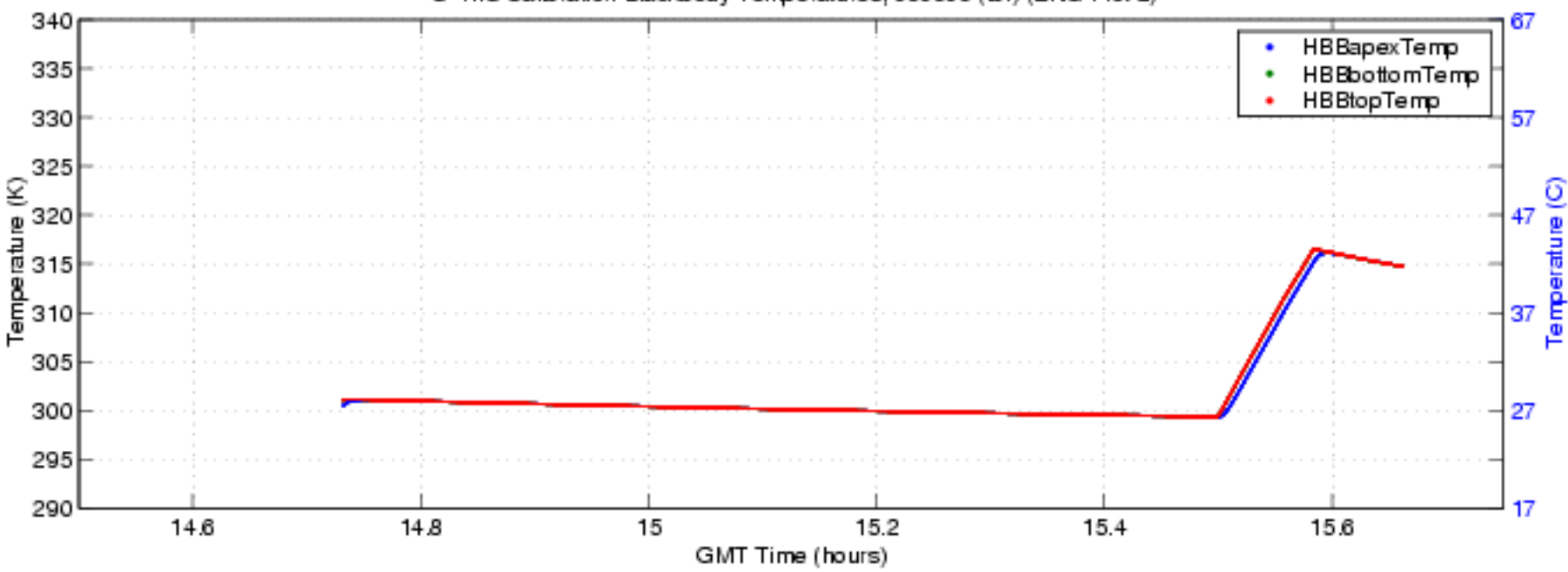
S-HIS Calibration Blackbody Temperatures, 050808 (bf) (ENG Plot 2)
